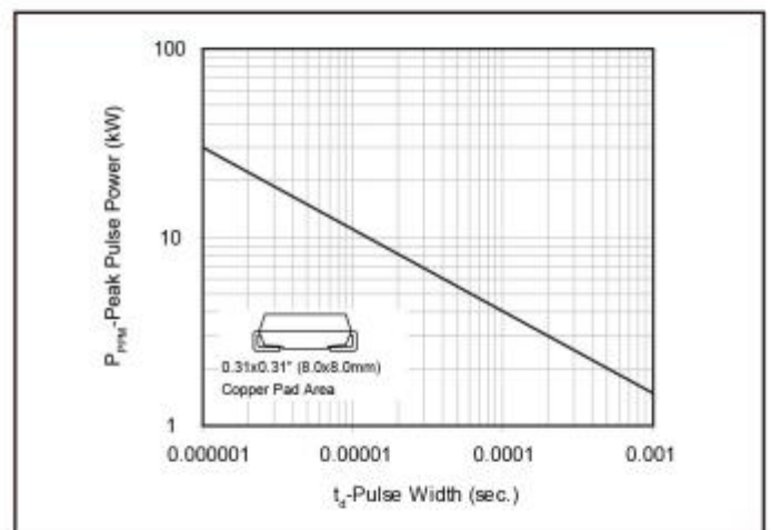
Figure 2 - Peak Pulse Power Rating
